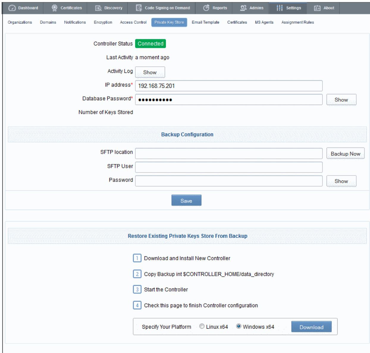
Private Key Store Interface - Table of Fields and Controls
